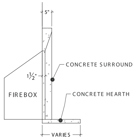
SECTION @ FIREBOX
