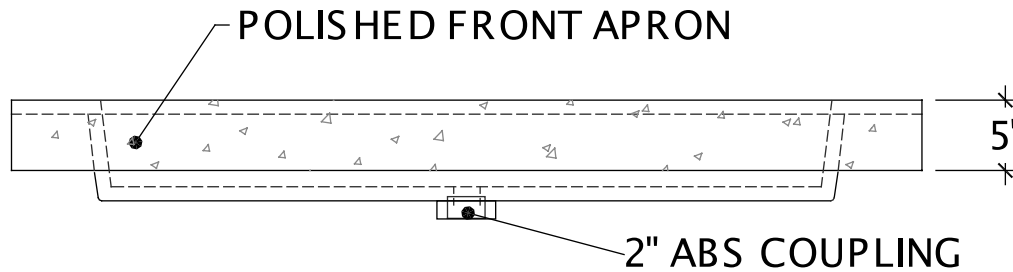
FRONT ELEVATION
