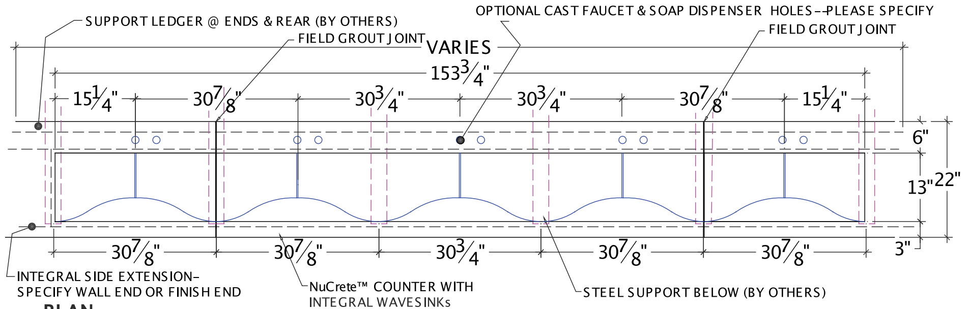
PLAN
