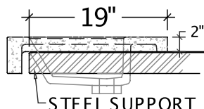
SECTION A
