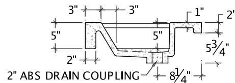
SECTION B
