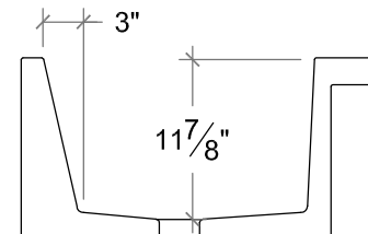
SIDE, APRON FRONT
