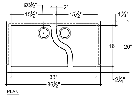
FS-CHEF-1633-L FRONT ELEVATION
