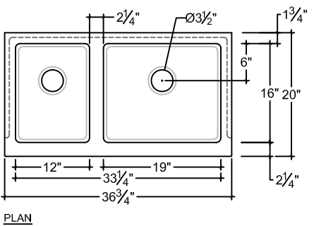
FS-DBL-1612-19 FRONT ELEVATION
