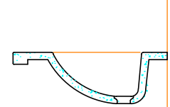
OVAL SINK SECTION W/ OFFSET DRAIN
