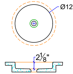
CS-12D-FB ♿ 12" DIA. x 2 1/8" DEEP
