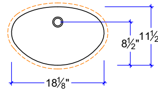
CS-1811* 18 1/8" x 11 1/2" x 5 7/8" 3 molds (enquire)
