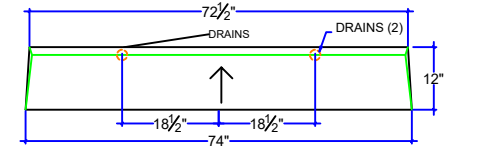
MOLD PLAN FRONT ELEVATION 6810-B SIDE
