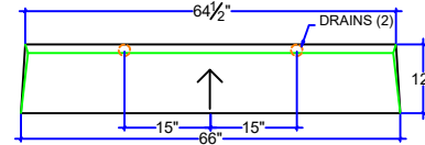
PLAN FRONT 4715-B (2) SIDE
