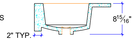
SECTION @ DRAIN
