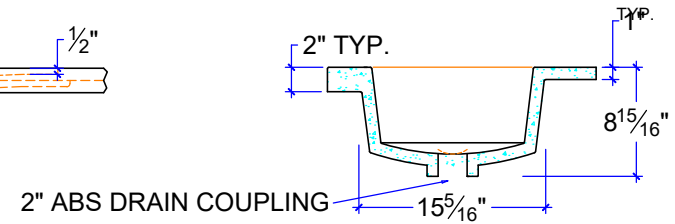
SECTION @ DRAIN
