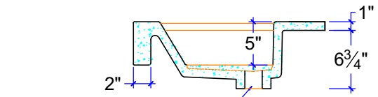
SECTION A
