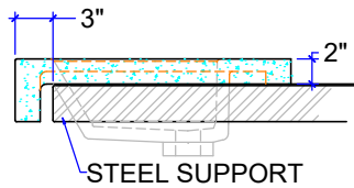
SECTION A
