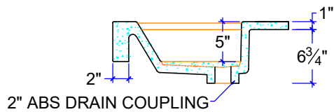
SECTION B
