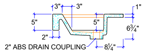
SECTION B
