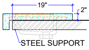
SECTION A
