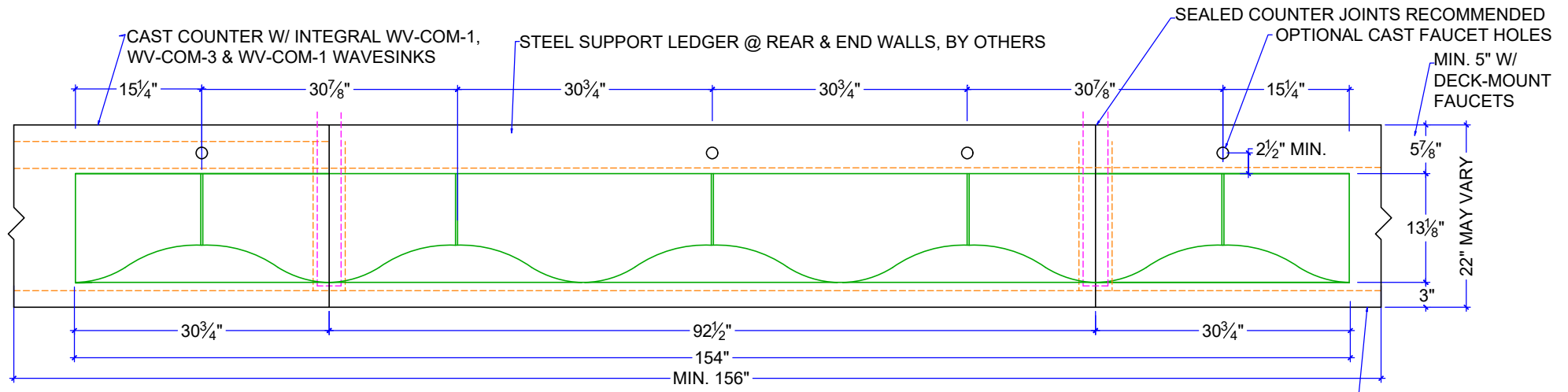
PLAN
