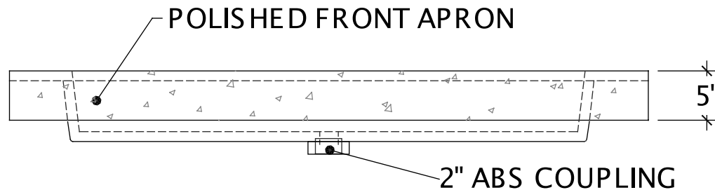
FRONT ELEVATION
