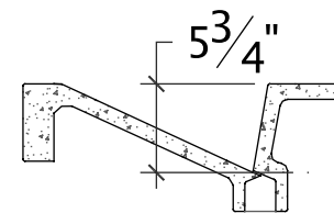
SECTION @ DRAIN
