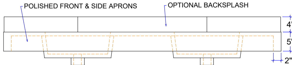
FRONT ELEVATION
