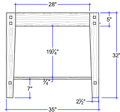
FRONT ELEVATION
