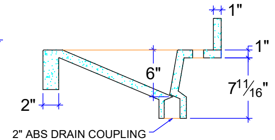
SECTION @ DRAIN
