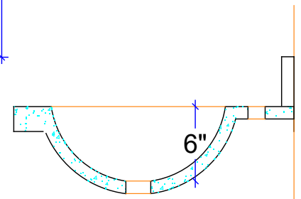
SECTION @ DRAIN
