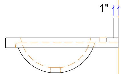
SECTION @ DRAIN
