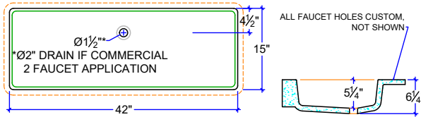
TYP. SIDE SECTION
